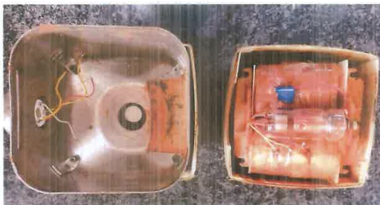
Teaching Model of Dismantled X-ray tube head
